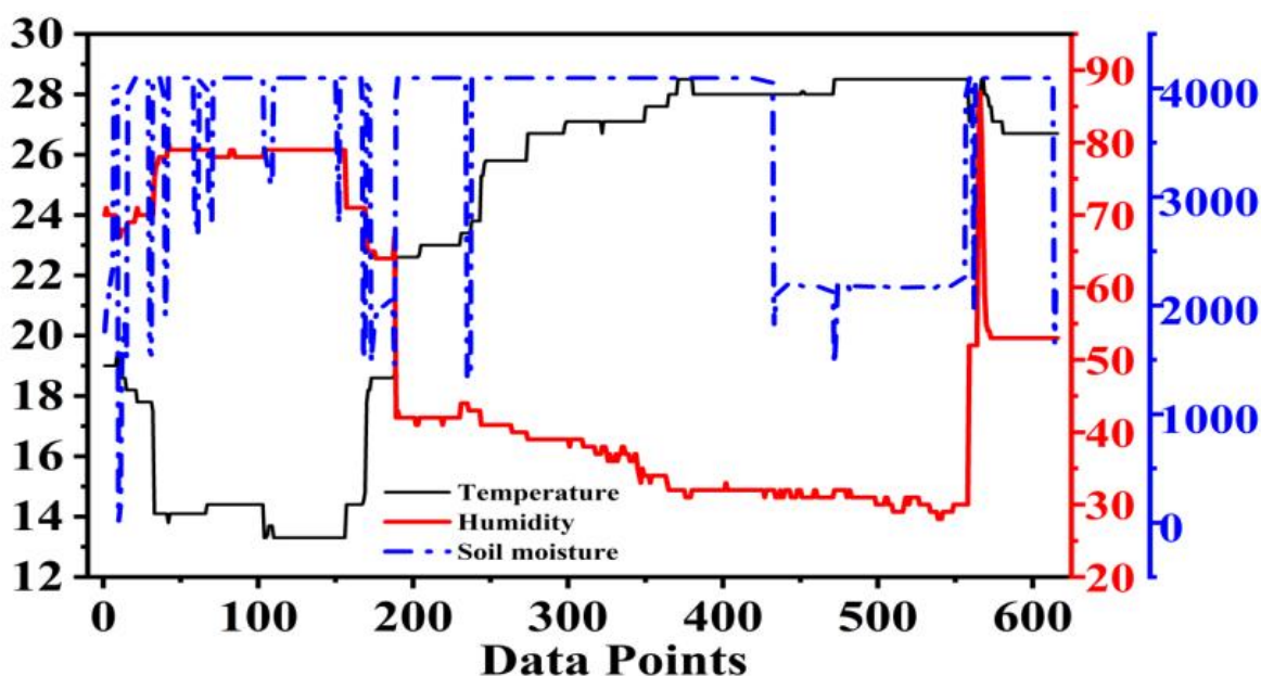
Figure 5. Temperature, humidity and soil moisture as a function of different data points.
